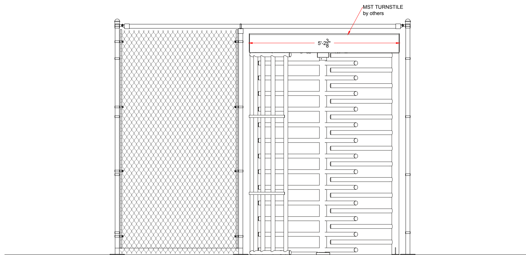
FRONT ELEVATION
